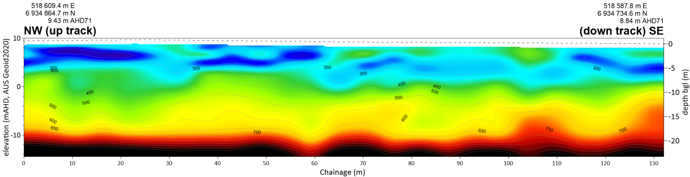
Seismic Line MASW AU-GP 185
